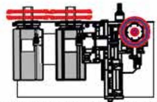
ST3 – One bottom horizontal scoring motor, plus two automatic vertical tool-motors
