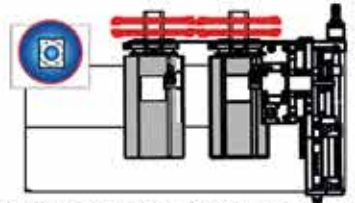
ST2 – Two automatic vertical tool-motors with Micro-bevel laquering unit.
